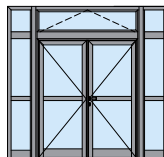
composite frame Door, 2-leaf inward or outward opening
